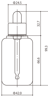
HB040-RO/UL-DROPPER
