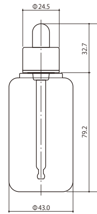
HB060-RO/UL-DROPPER
