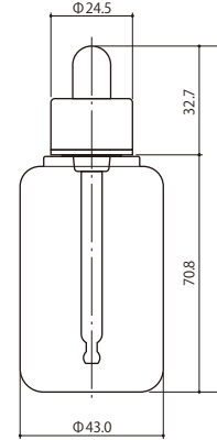
HB050-RO/UL-DROPPER
