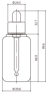
HB030-RO/UL-DROPPER
