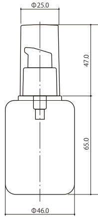
HB060-RO/UL-T
