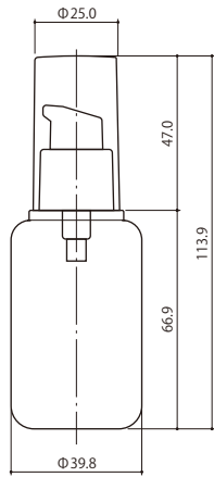
HB030-RO/UL-T
