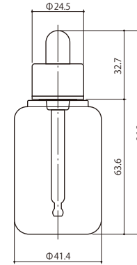
HB035-RO/UL-DROPPER
