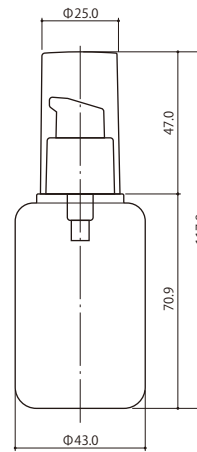
HB050-RO/UL-T
