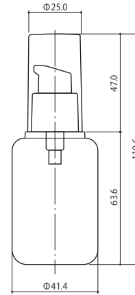
HB035-RO/UL-T
